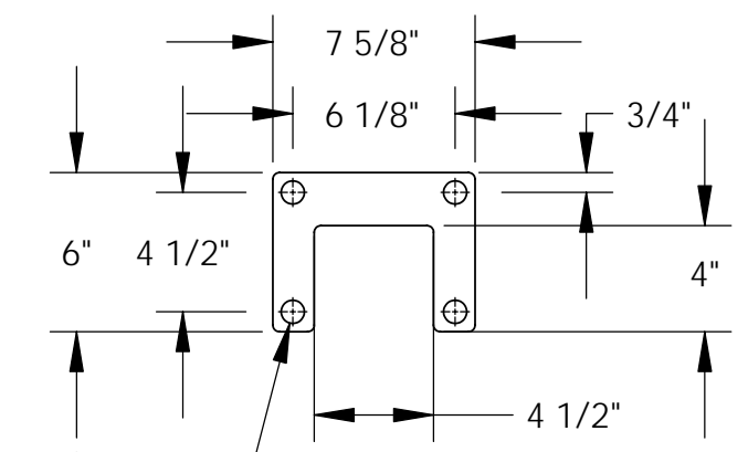
DETAIL VIEW OF MIDDLE MOUNT BRACKET
