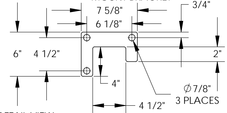
DETAIL VIEW OF END MOUNT BRACKET
